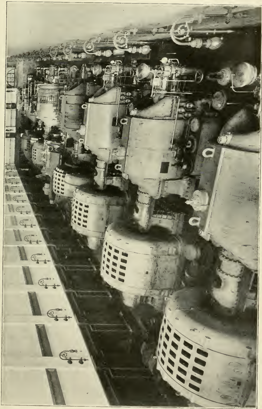
WESTINGHOUSE TUBRO-GENERATOR INSTALLATION OF THE BROOKLYN RAPID TRANSIT COMPANY. RATED CAPACITY OF PLANT 100,000 KILOWATTS
